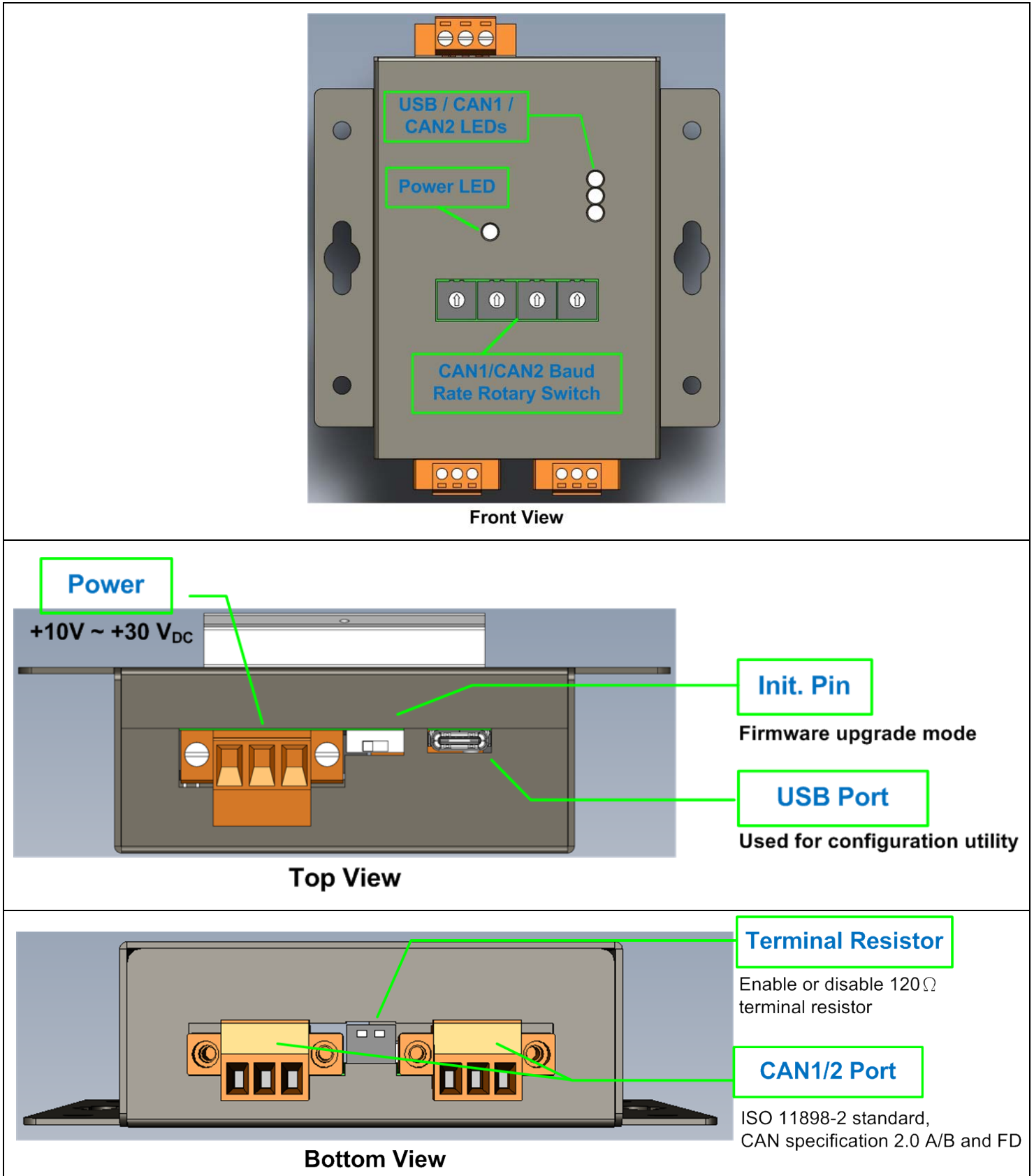
Figure 2-1-1 Appearance of I-7532RM-FD
