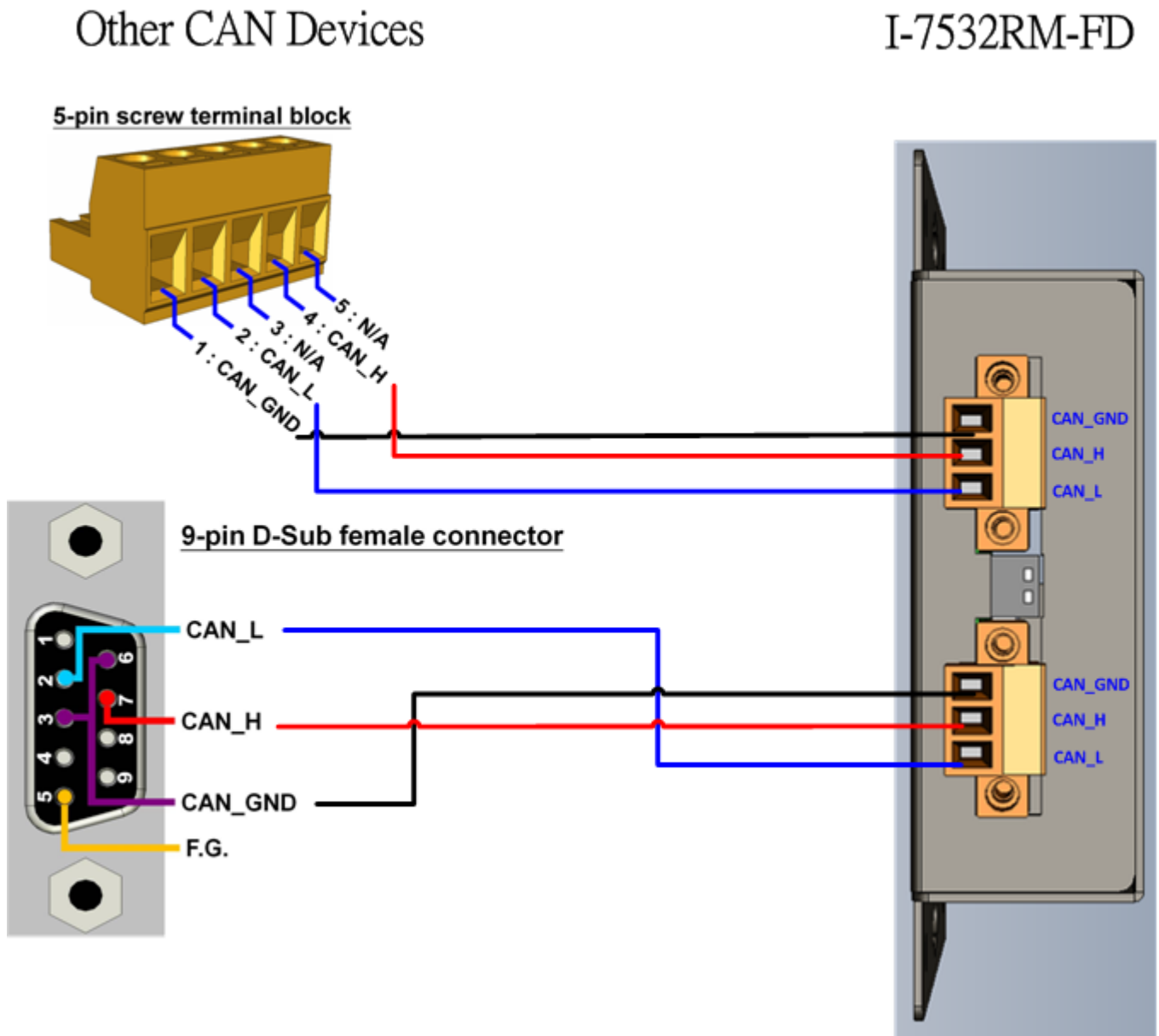
Figure 2-6-1 Wire Connection for I-7532RM-FD
