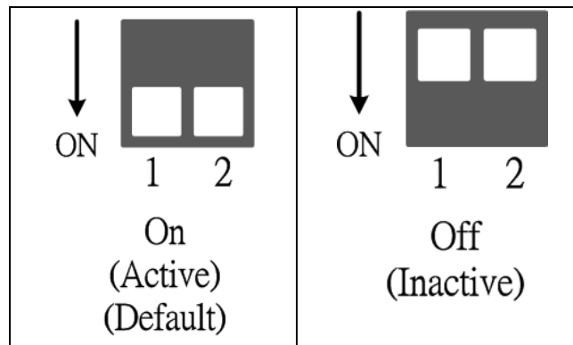
Figure 2-5-3 Adjustment of Terminal Resistance
