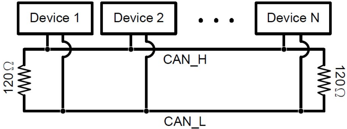
Figure 2-5-1 CAN bus network topology
