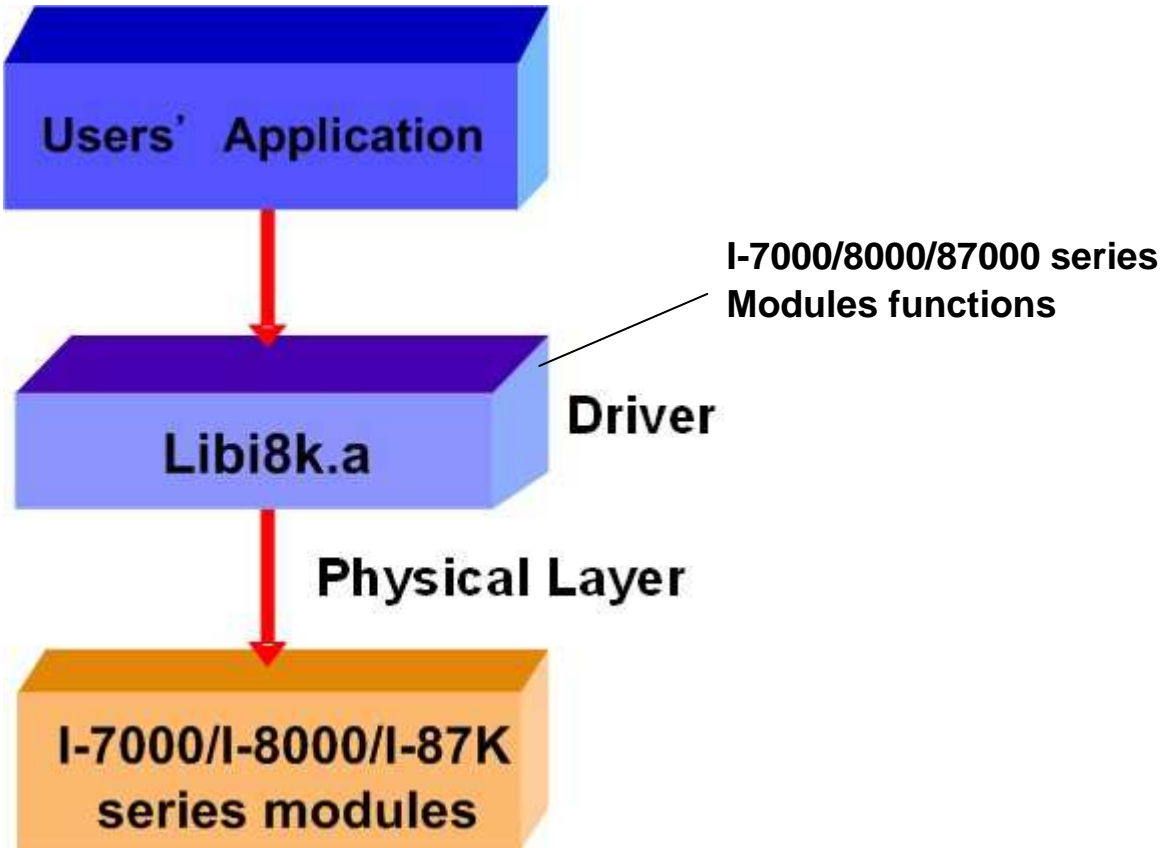
Fig. 3-1 Functions for LP-8X81 Embedded Controller are divided into sub-groups for
