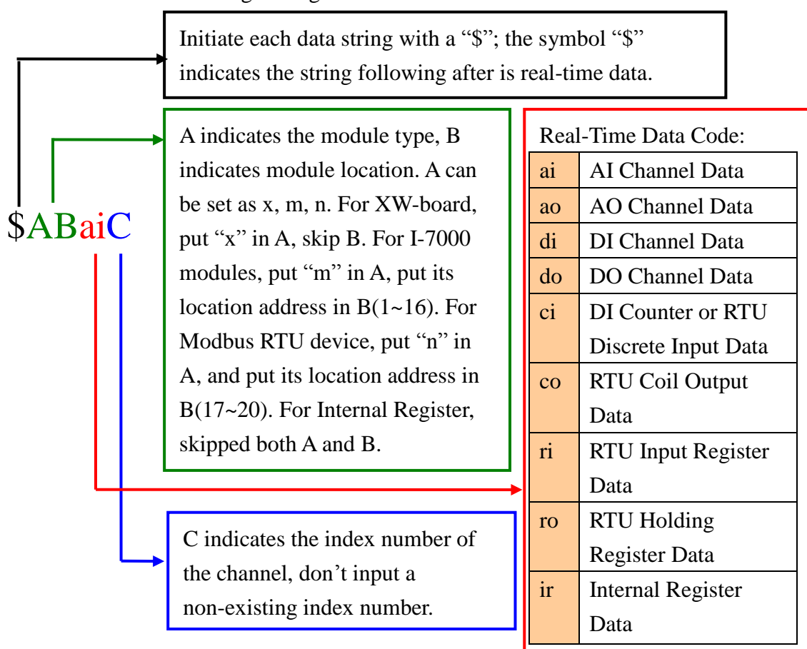
Figure 5-16 : SMS Command Data Retrieve Coding Rules
