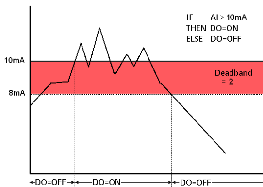
Figure 4-10 : AI Deadband Operation(> or >= a numerical value)
