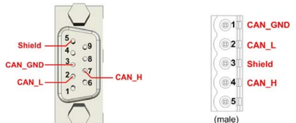
9 pin male D-sub connector 5 pin screw terminal connector
